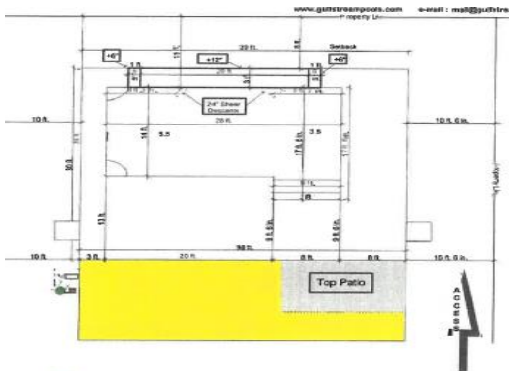
Construction Drawing (Location, Distance and Dimensions to Scale of Swimming Pool and Screen Enclosure)
